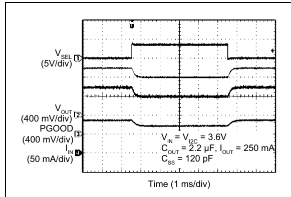
FIGURE 2-33: V_{OUT} During V_{SEL} Transition.
