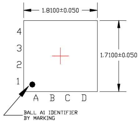
TOP VIEW NOTE: 1, 2
