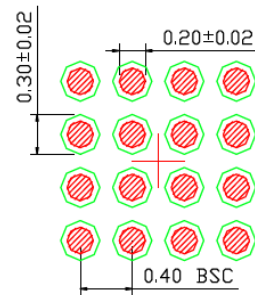
RECOMMENDED LAND PATTERN NOTE: 3, 4
