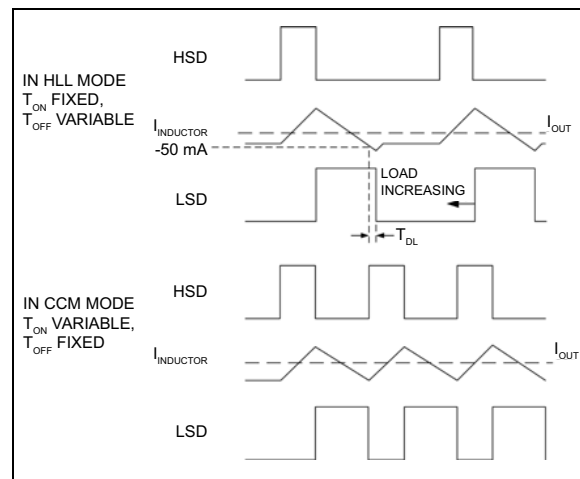
FIGURE 5-1: HSD Signals for t_{\text{ON}} Control, Inductor Current and LSD for t_{\text{OFF}} Control.
