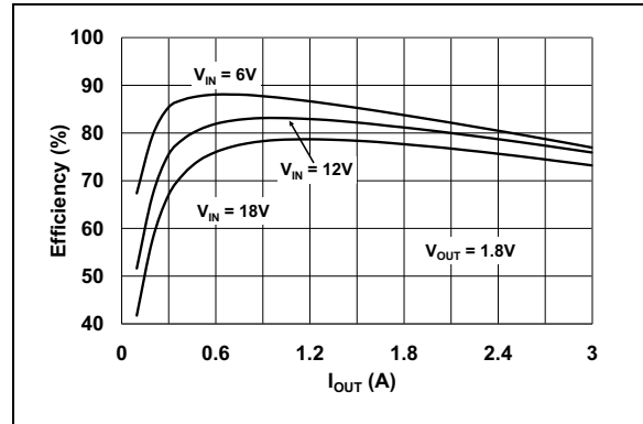
FIGURE 2-4: 1.8V V_{OUT} Efficiency vs. I_{OUT} .
